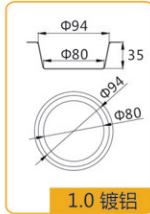
1.0 镀铝
