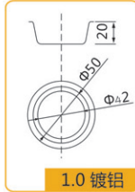
1.0 镀铝
