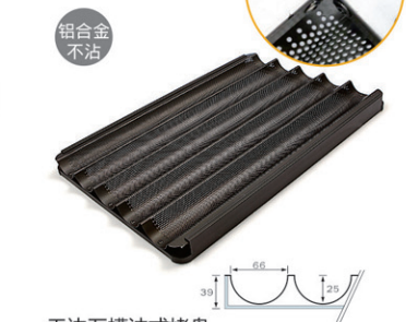
无边五槽法式烤盘 Non-stick French Bread Sheet Pan (5 Rows)
