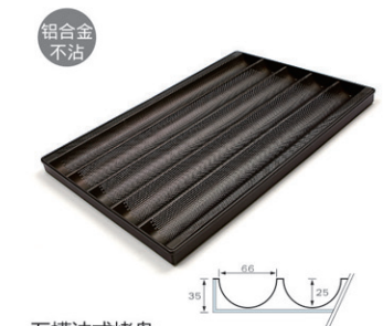
五槽法式烤盘 Non-stick French Bread Sheet Pan (5 Rows)
